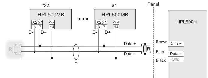
Figure 1 MODbus network
